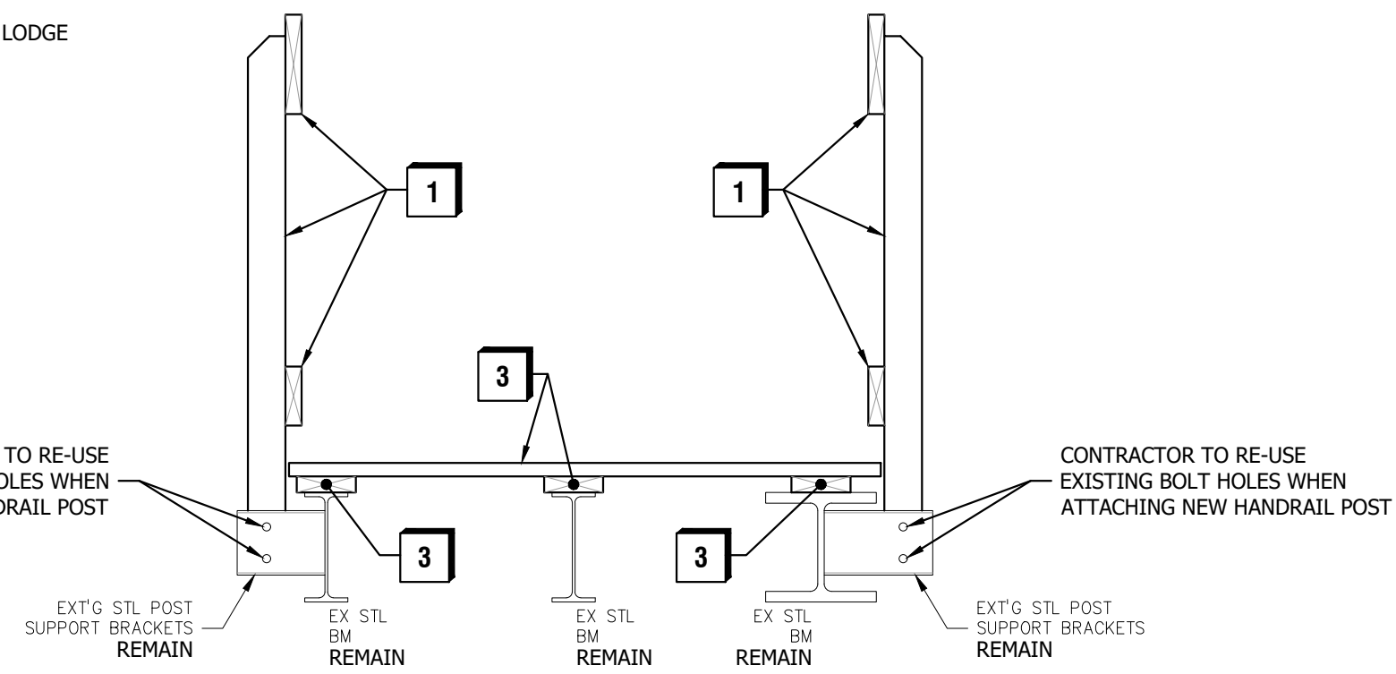
TYPICAL EXISTING BRIDGE CROSS-SECTION
